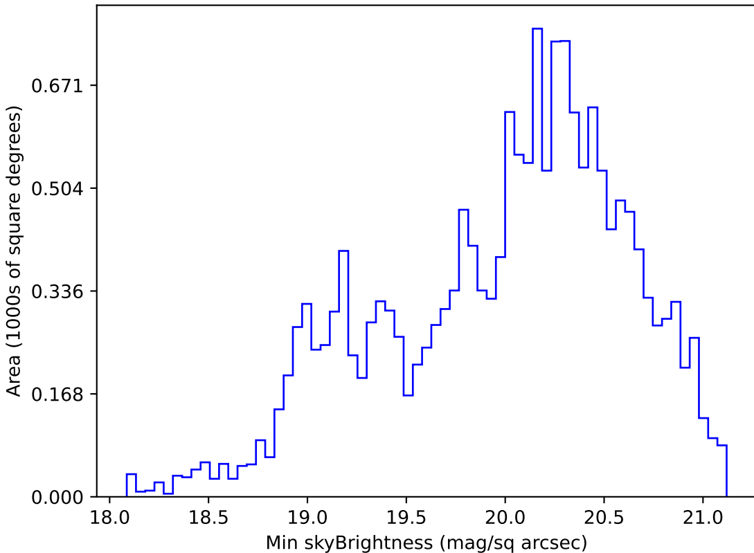
extra_ss_neo4_v3.4_10yrs WFD g band: Min skyBrightness
