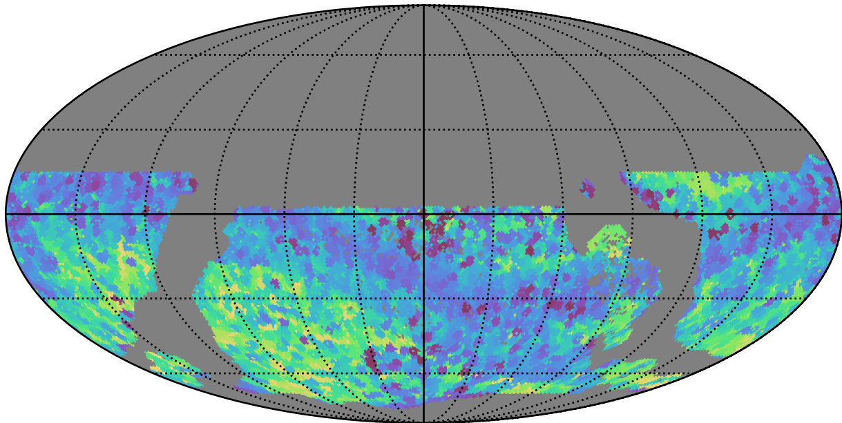
extra_ss_neo4_v3.4_10yrs WFD all bands: Min skyBrightness
