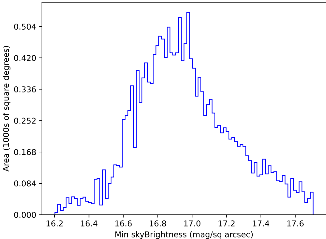
extra_ss_neo4_v3.4_10yrs WFD all bands: Min skyBrightness
