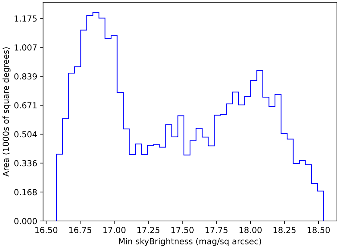
extra_ss_neo4_v3.4_10yrs All sky z band: Min skyBrightness
