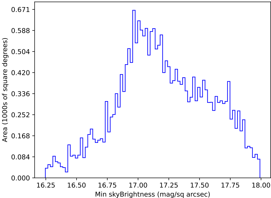
extra_ss_neo4_v3.4_10yrs All sky y band: Min skyBrightness
