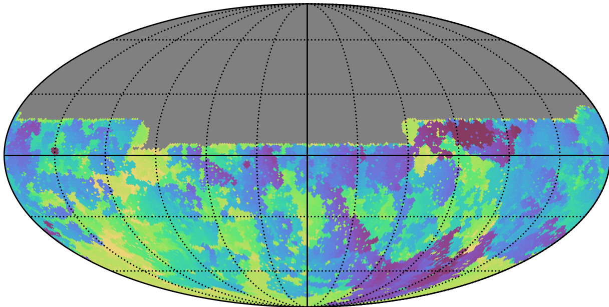
extra_ss_neo4_v3.4_10yrs All sky u band: Min skyBrightness
