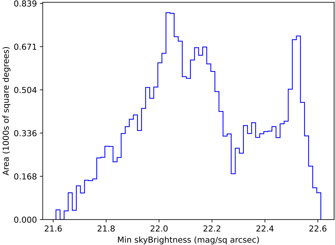
extra_ss_neo4_v3.4_10yrs All sky u band: Min skyBrightness
