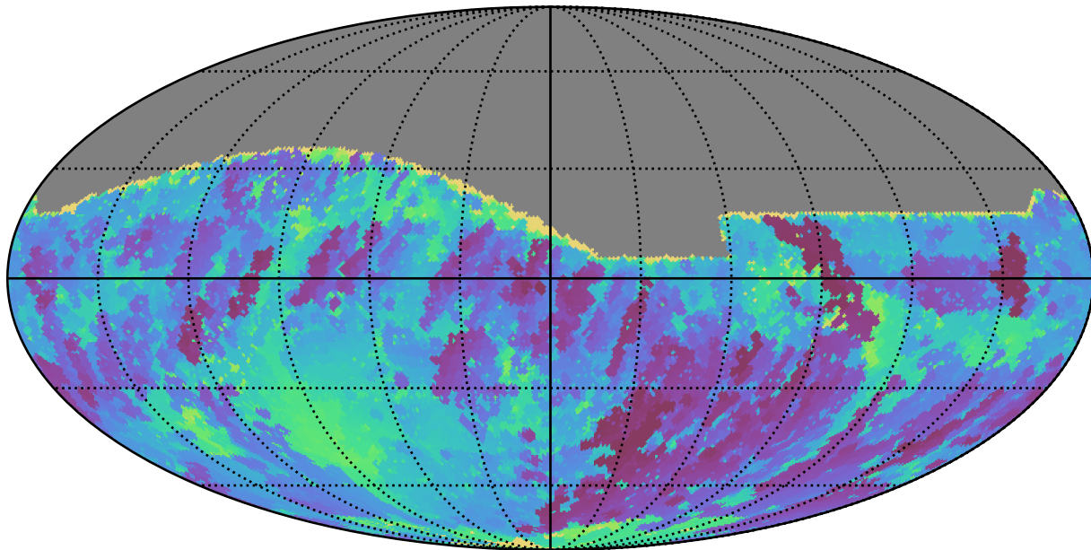
extra_ss_neo4_v3.4_10yrs All sky r band: Min skyBrightness
