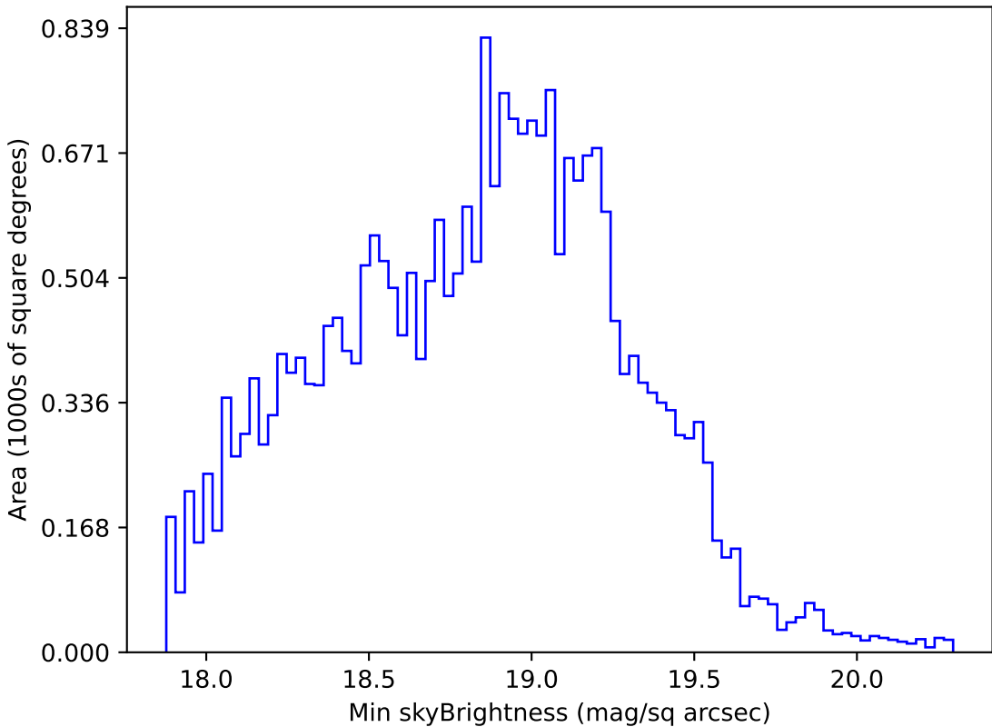
extra_ss_neo4_v3.4_10yrs All sky r band: Min skyBrightness
