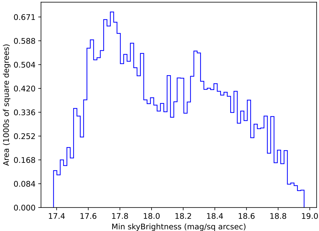
extra_ss_neo4_v3.4_10yrs All sky i band: Min skyBrightness
