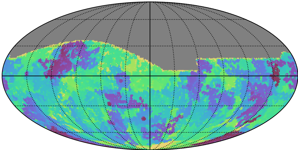
extra_ss_neo4_v3.4_10yrs All sky g band: Min skyBrightness
