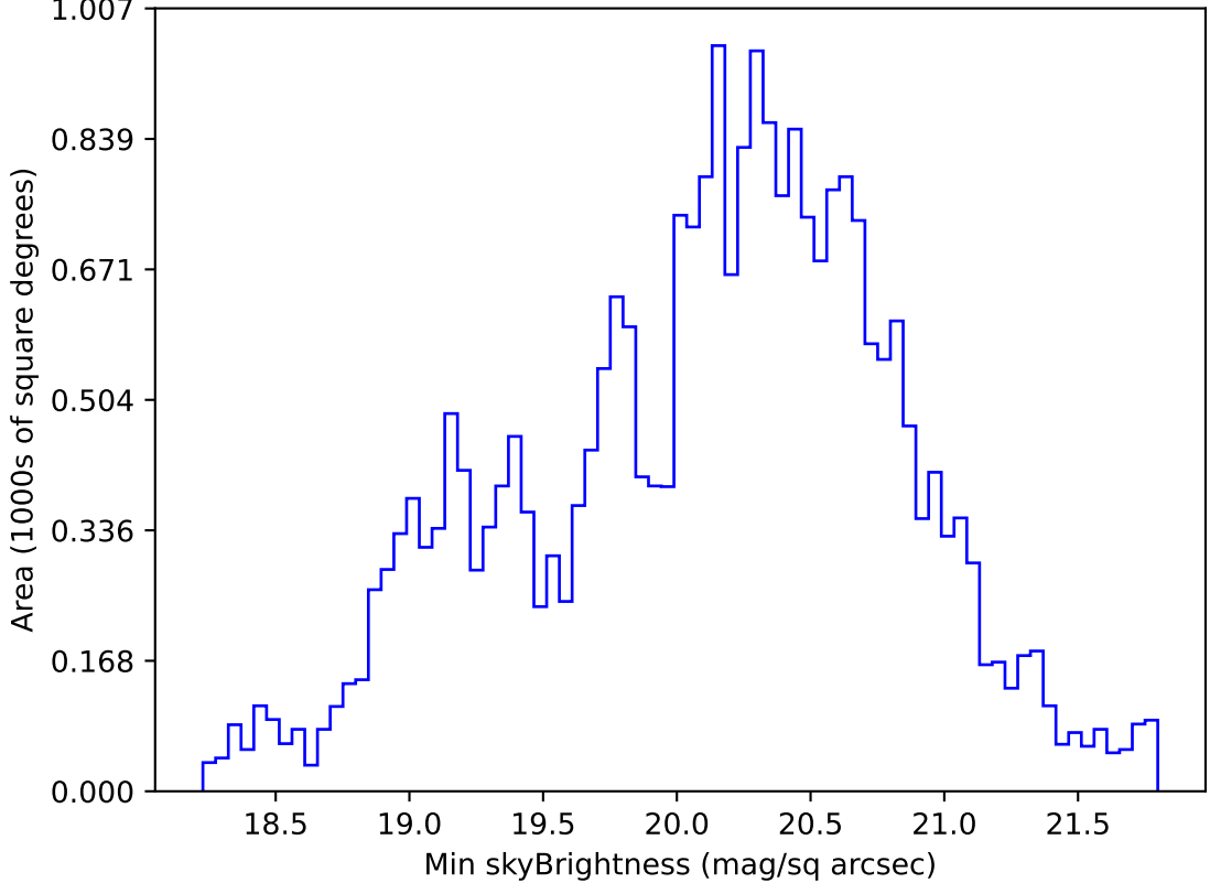
extra_ss_neo4_v3.4_10yrs All sky g band: Min skyBrightness
