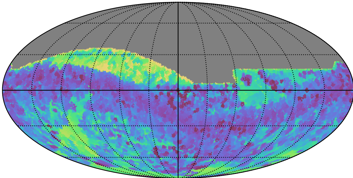
extra_ss_neo4_v3.4_10yrs All sky all bands: Min skyBrightness
