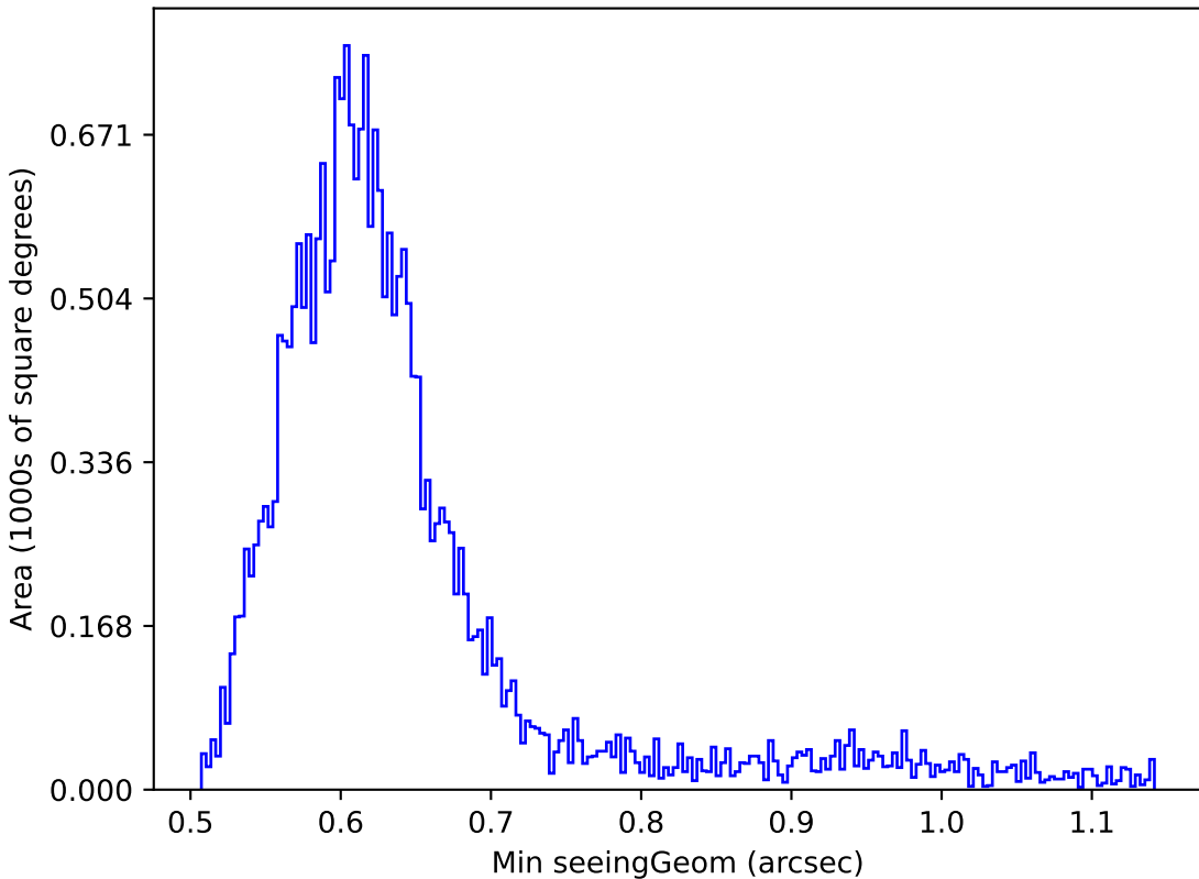
extra_ss_neo4_v3.4_10yrs Yr 1 r band: Min seeingGeom
