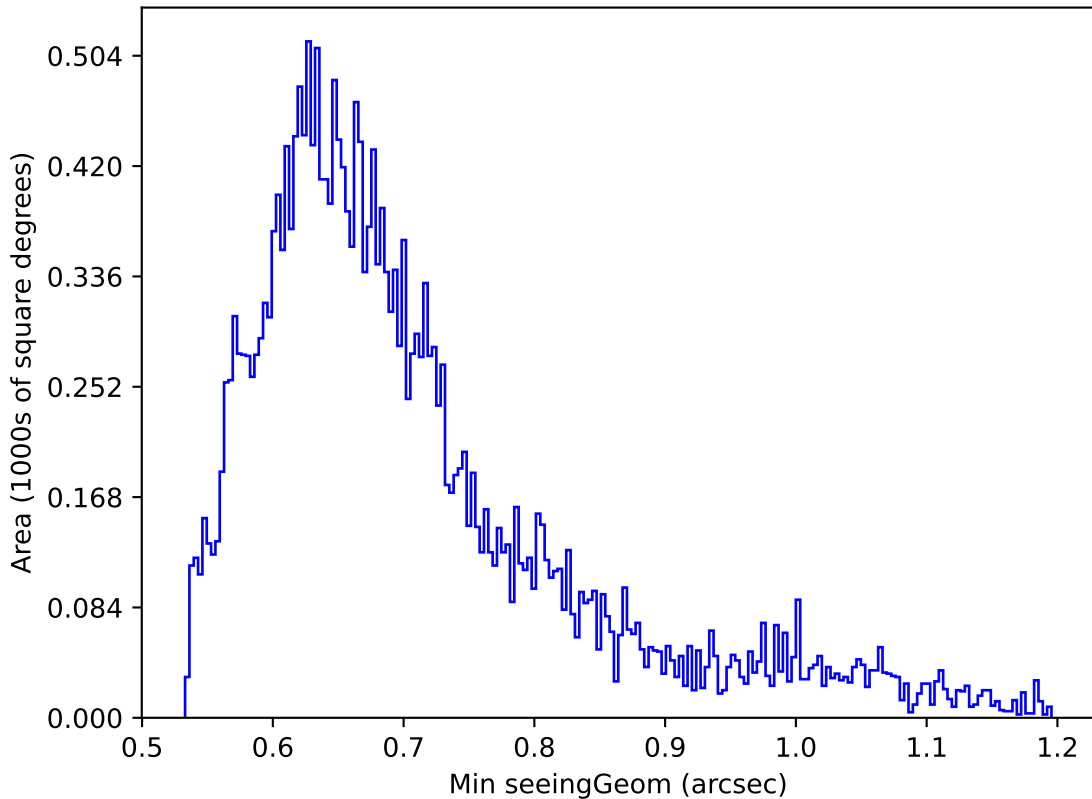
extra_ss_neo4_v3.4_10yrs Yr 1 g band: Min seeingGeom
