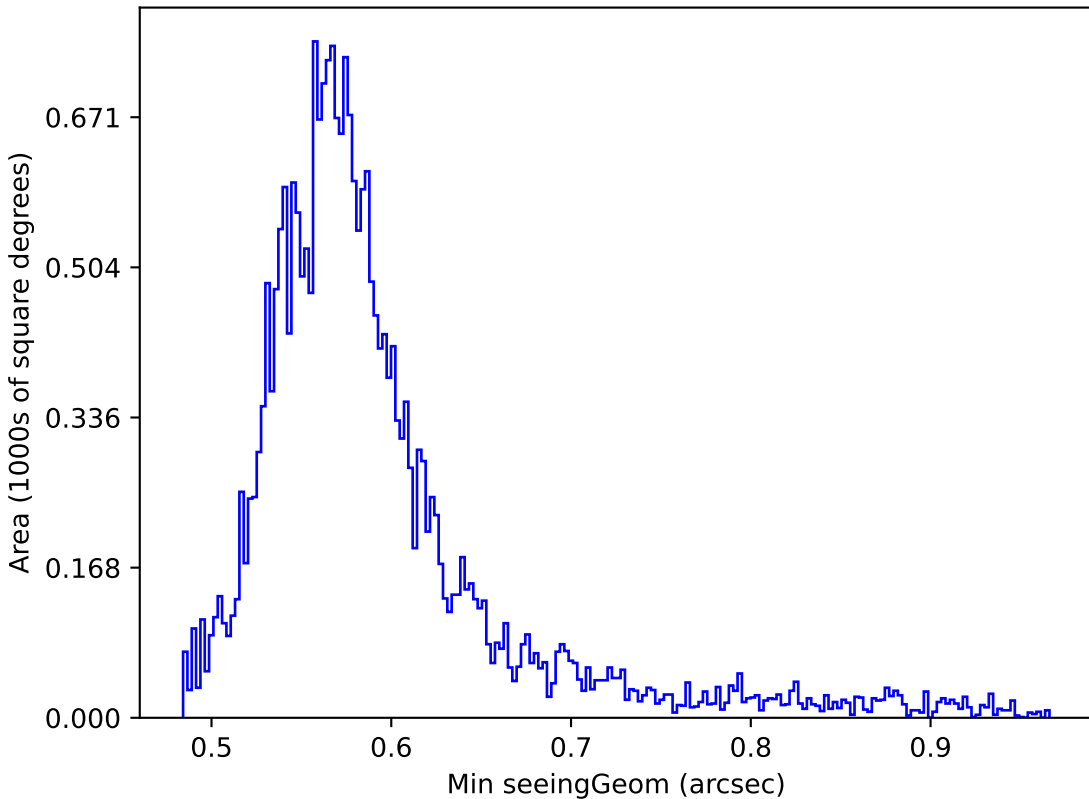
extra_ss_neo4_v3.4_10yrs Yr 1 all bands: Min seeingGeom
