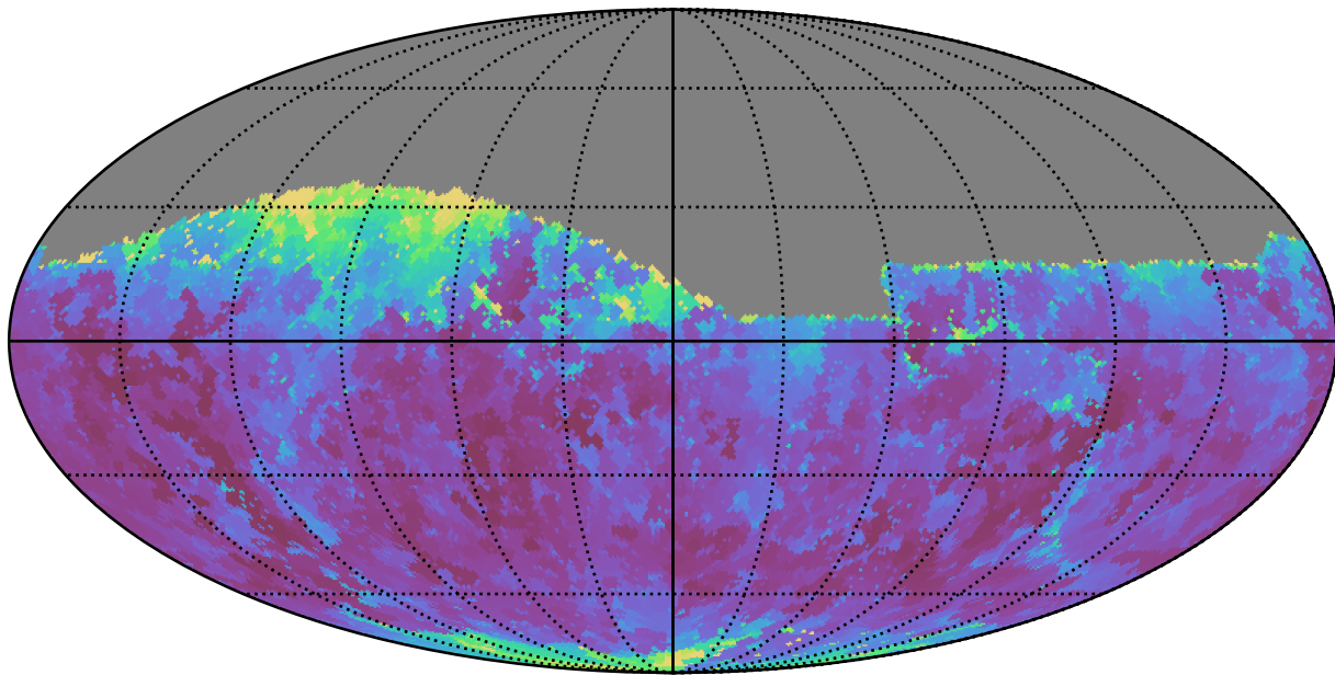
extra_ss_neo4_v3.4_10yrs Yr 1 z band: Min seeingEff
