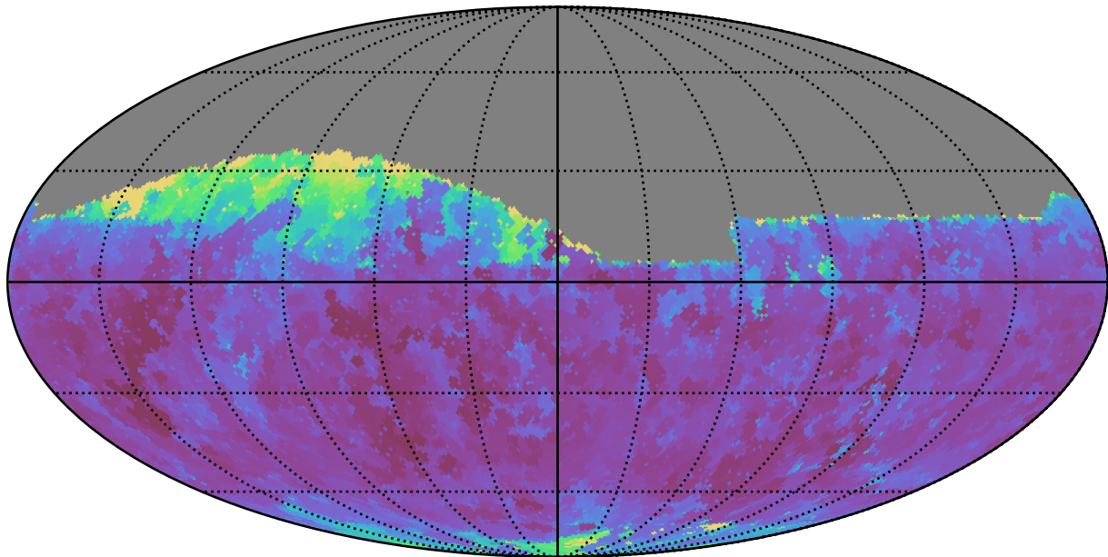
extra_ss_neo4_v3.4_10yrs Yr 1 i band: Min seeingEff
