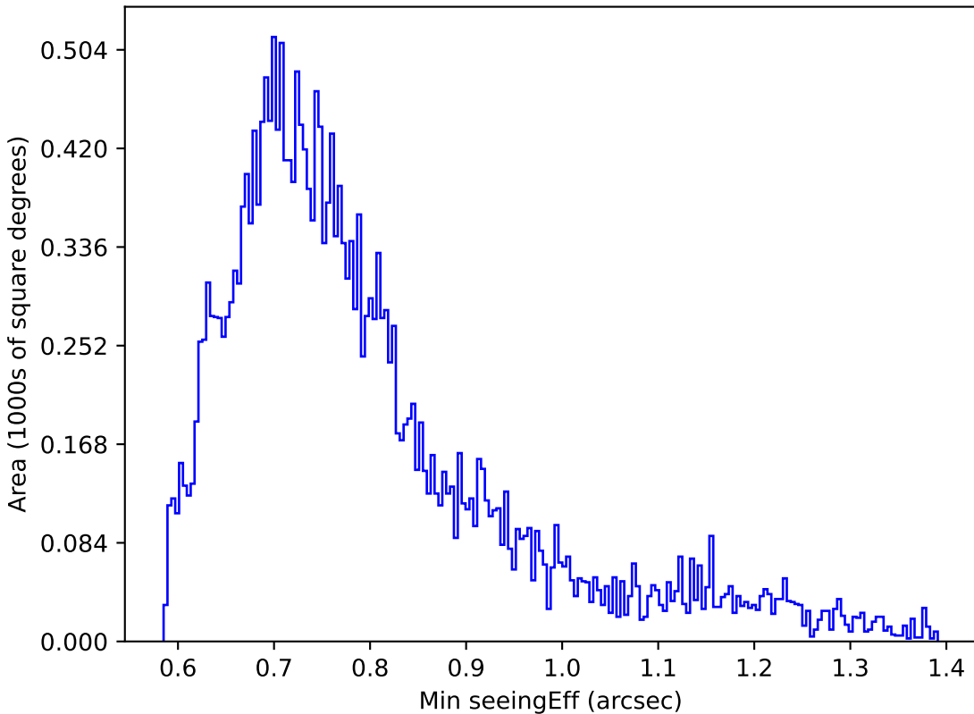
extra_ss_neo4_v3.4_10yrs Yr 1 g band: Min seeingEff
