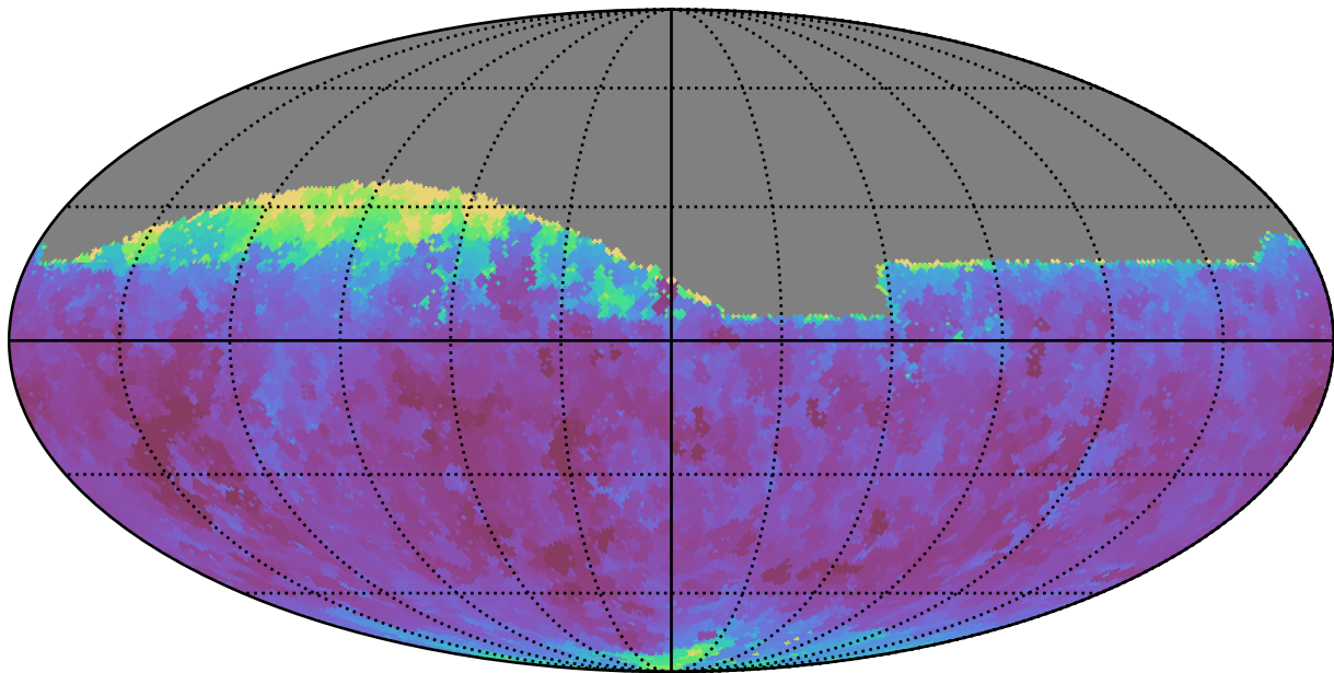
extra_ss_neo4_v3.4_10yrs Yr 1 all bands: Min seeingEff
