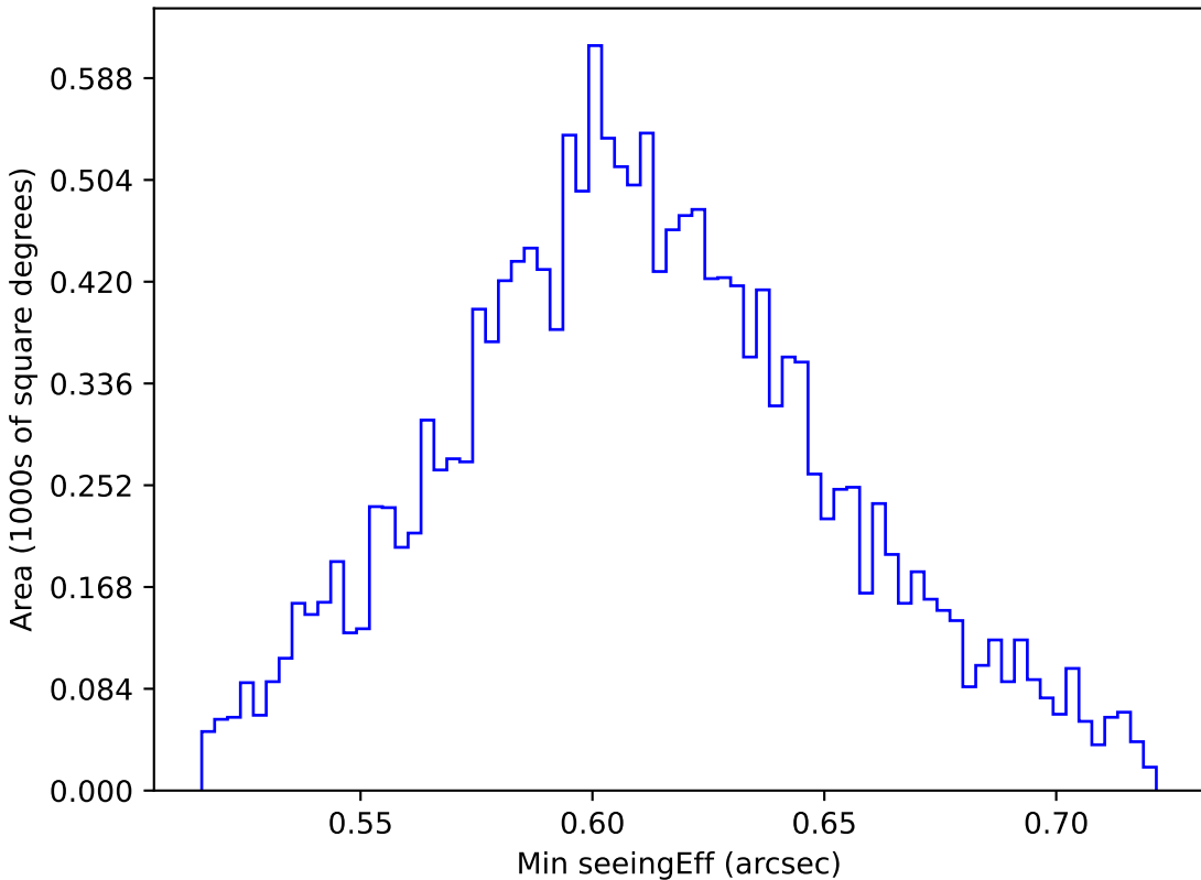
extra_ss_neo4_v3.4_10yrs WFD z band: Min seeingEff
