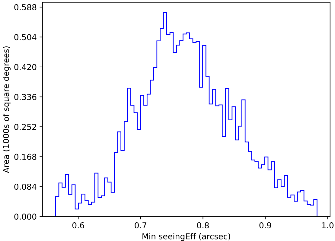
extra_ss_neo4_v3.4_10yrs WFD u band: Min seeingEff
