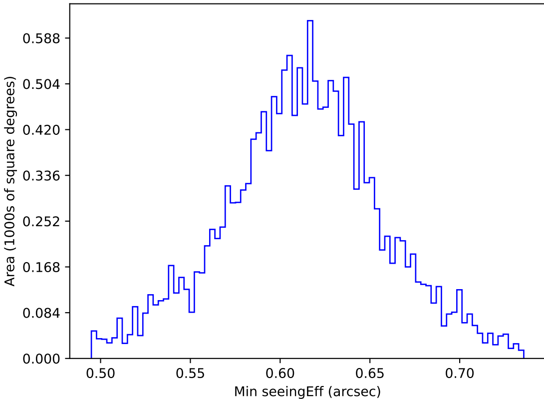
extra_ss_neo4_v3.4_10yrs WFD r band: Min seeingEff
