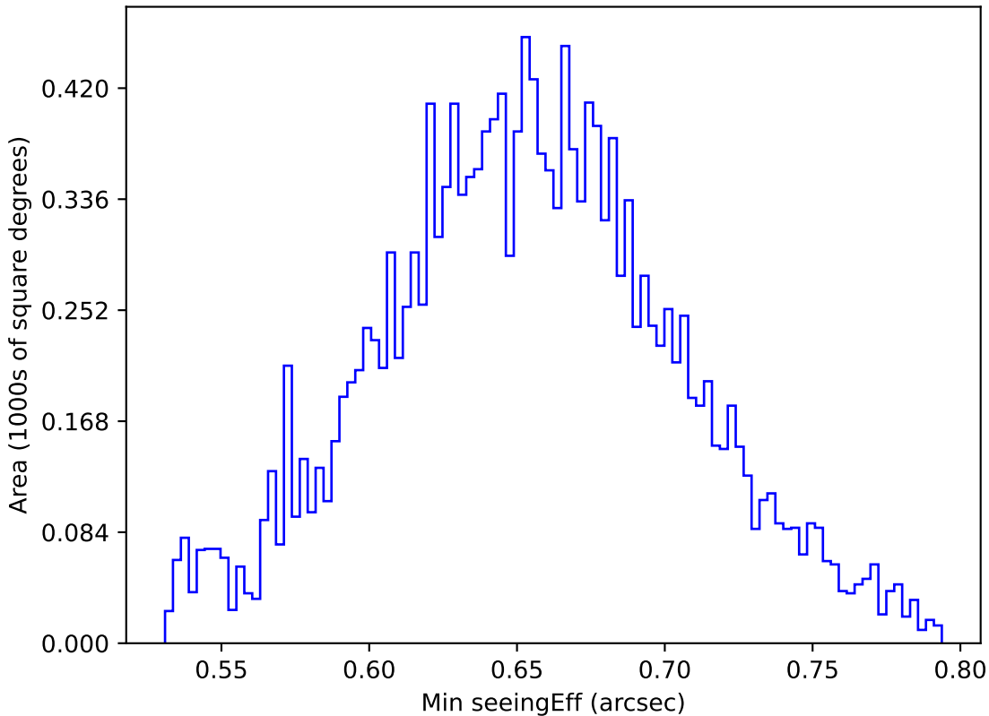
extra_ss_neo4_v3.4_10yrs WFD g band: Min seeingEff
