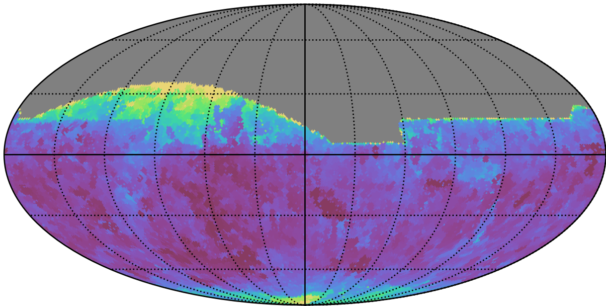
extra_ss_neo4_v3.4_10yrs All sky z band: Min seeingEff
