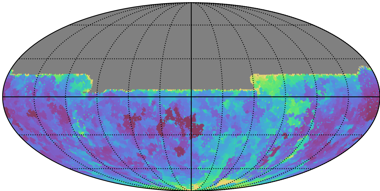
extra_ss_neo4_v3.4_10yrs All sky u band: Min seeingEff
