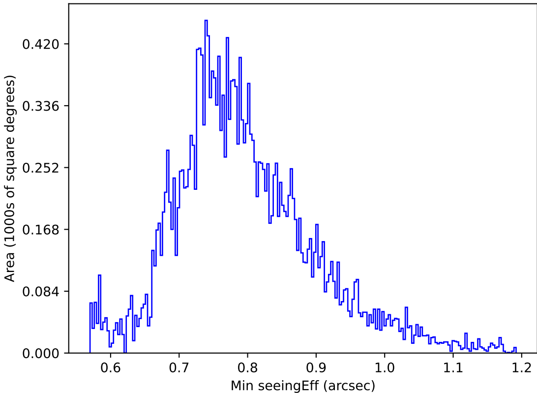
extra_ss_neo4_v3.4_10yrs All sky u band: Min seeingEff
