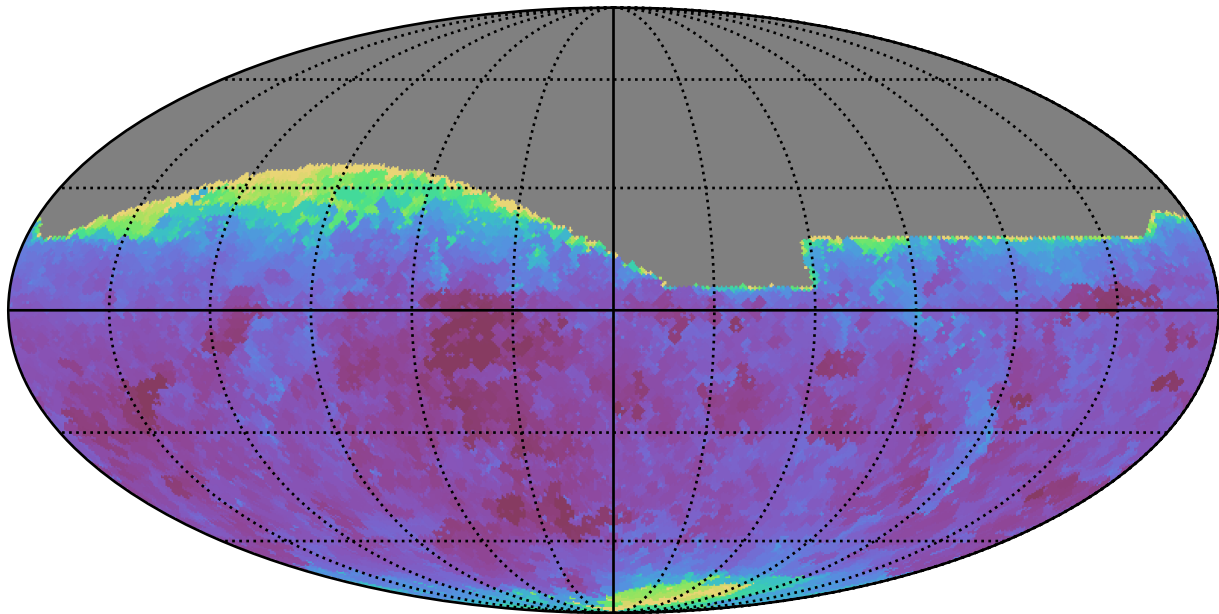
extra_ss_neo4_v3.4_10yrs All sky r band: Min seeingEff
