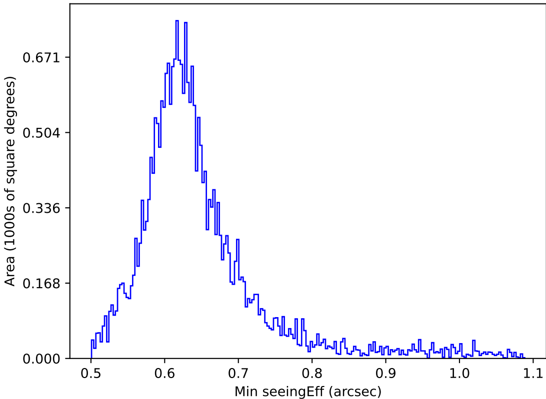
extra_ss_neo4_v3.4_10yrs All sky r band: Min seeingEff
