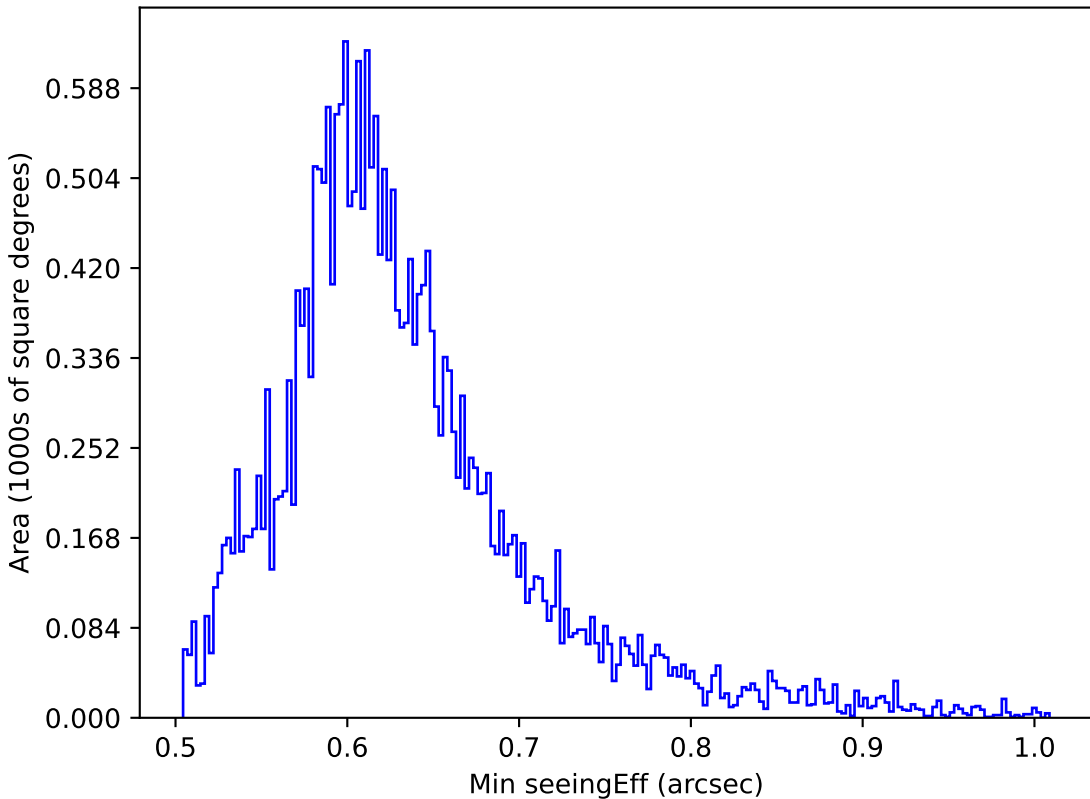
extra_ss_neo4_v3.4_10yrs All sky i band: Min seeingEff
