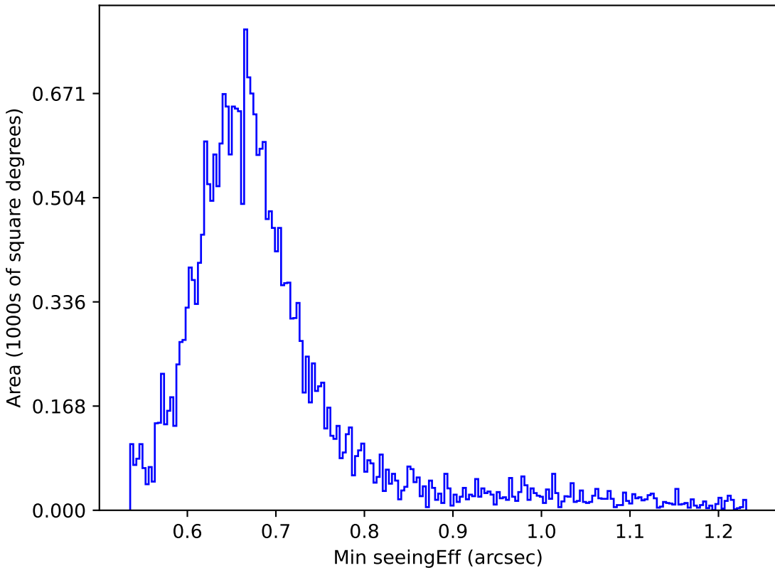
extra_ss_neo4_v3.4_10yrs All sky g band: Min seeingEff
