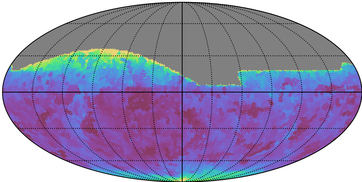
extra_ss_neo4_v3.4_10yrs All sky all bands: Min seeingEff
