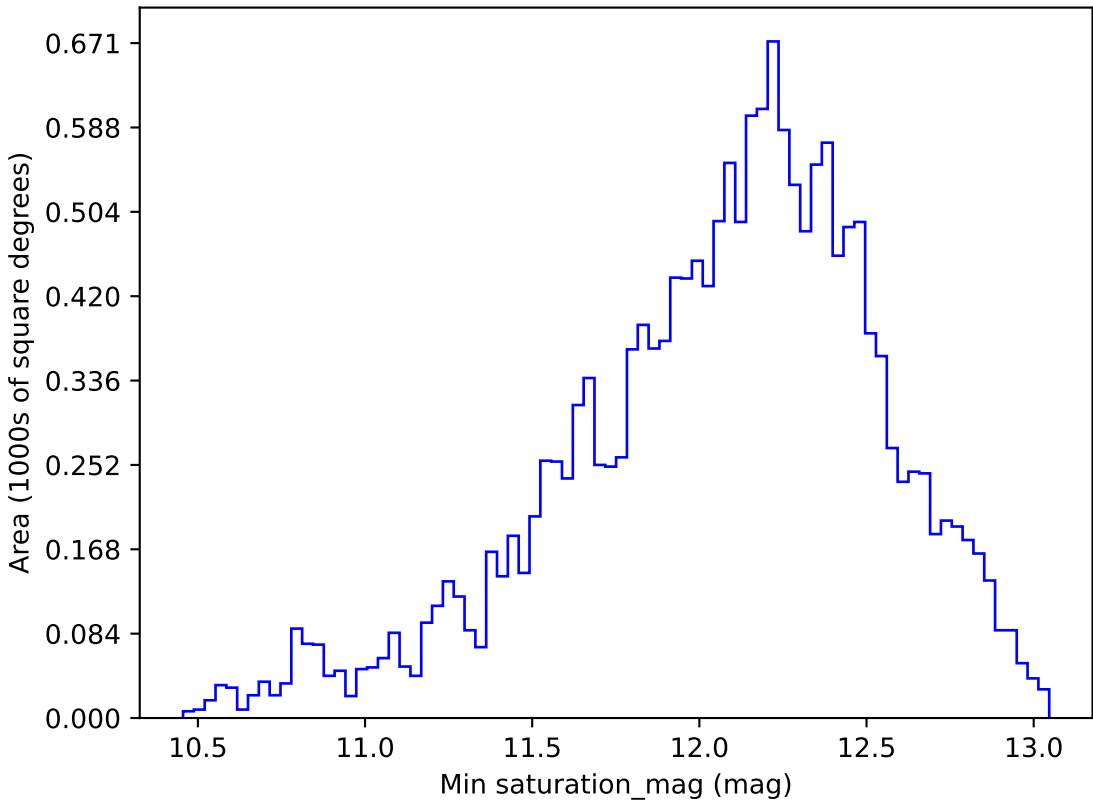
extra_ss_neo4_v3.4_10yrs WFD z band: Min saturation_mag
