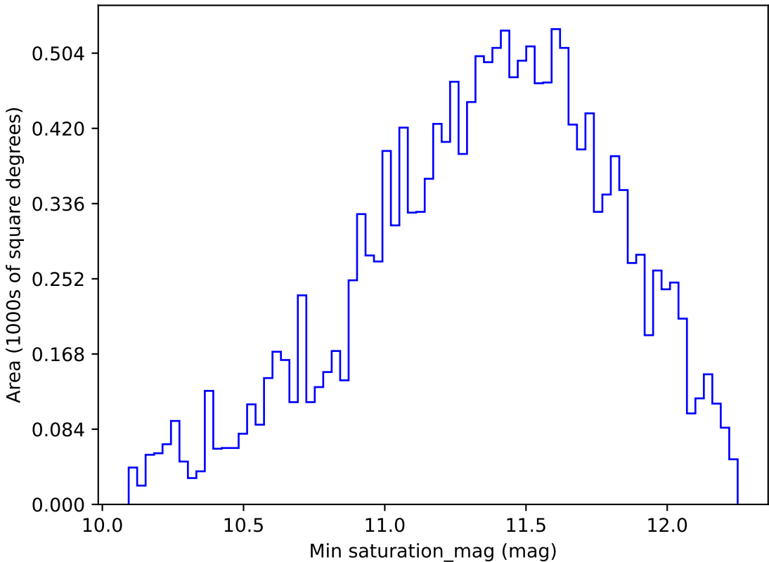
extra_ss_neo4_v3.4_10yrs WFD u band: Min saturation_mag
