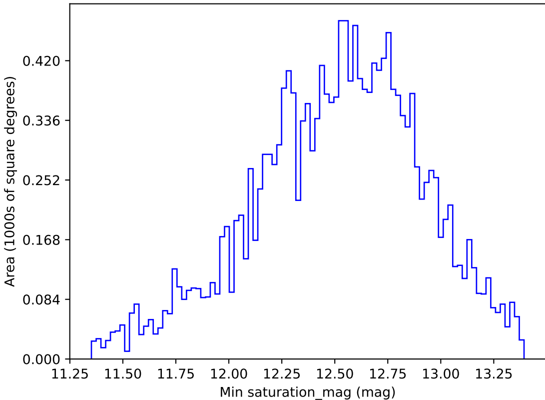
extra_ss_neo4_v3.4_10yrs WFD r band: Min saturation_mag
