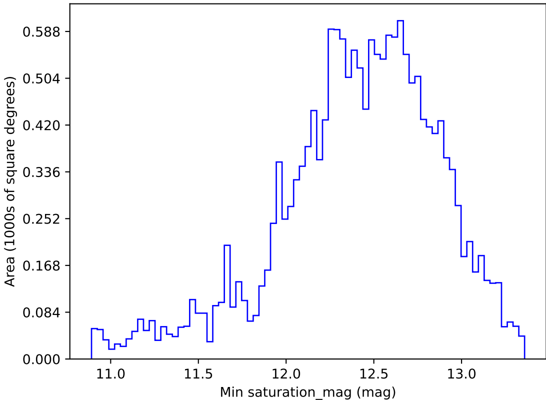
extra_ss_neo4_v3.4_10yrs WFD i band: Min saturation_mag
