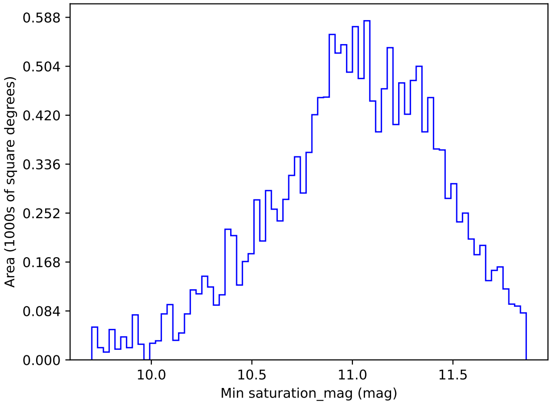
extra_ss_neo4_v3.4_10yrs WFD all bands: Min saturation_mag
