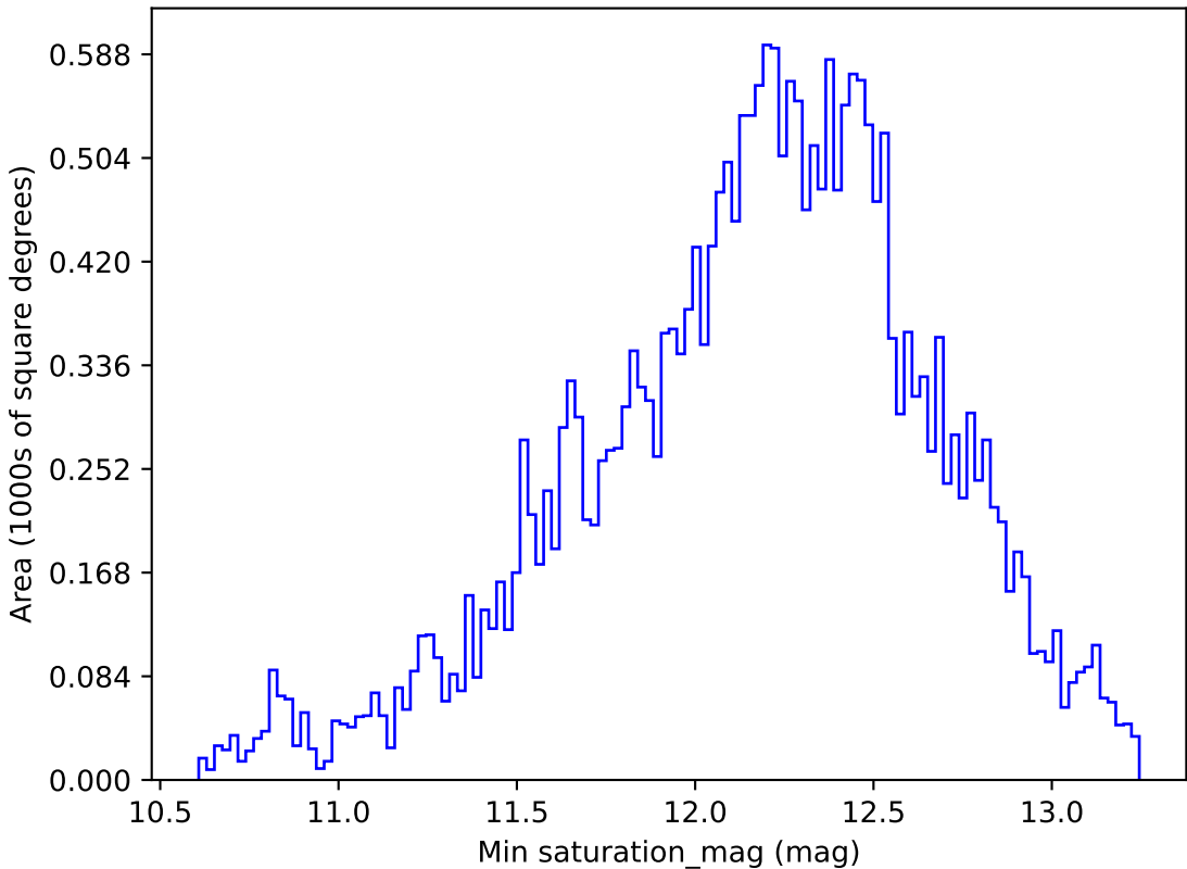
extra_ss_neo4_v3.4_10yrs All sky z band: Min saturation_mag
