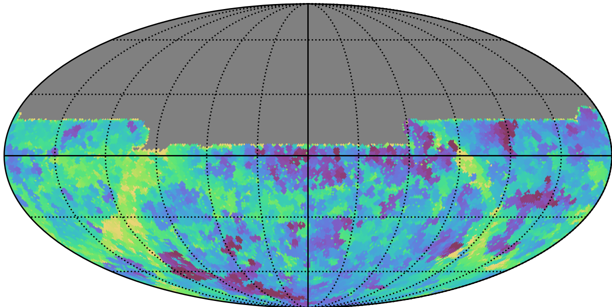
extra_ss_neo4_v3.4_10yrs All sky u band: Min saturation_mag
