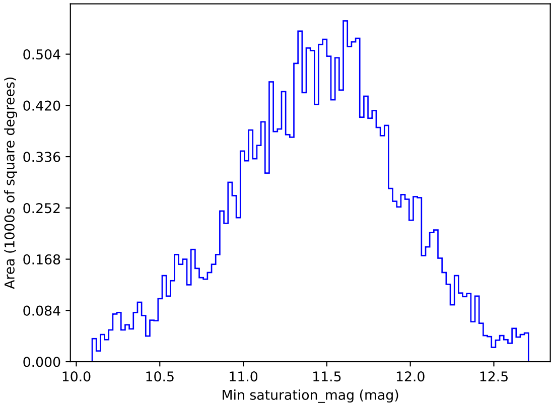
extra_ss_neo4_v3.4_10yrs All sky u band: Min saturation_mag
