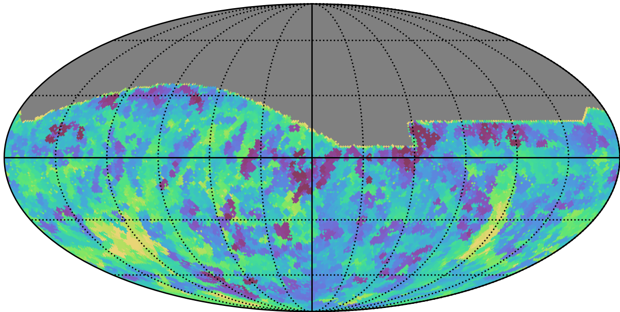
extra_ss_neo4_v3.4_10yrs All sky r band: Min saturation_mag
