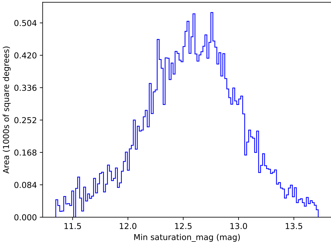
extra_ss_neo4_v3.4_10yrs All sky r band: Min saturation_mag
