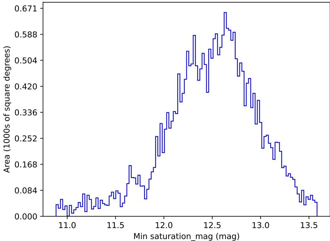
extra_ss_neo4_v3.4_10yrs All sky i band: Min saturation_mag
