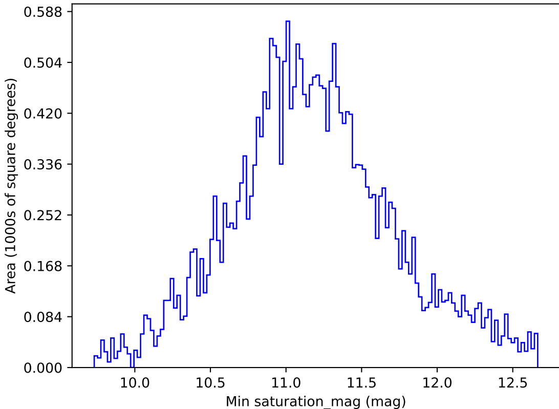
extra_ss_neo4_v3.4_10yrs All sky all bands: Min saturation_mag
