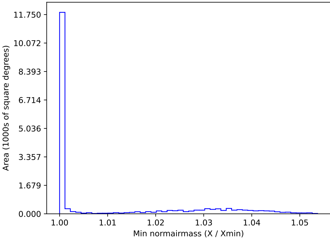
extra_ss_neo4_v3.4_10yrs WFD u band: Min normairmass
