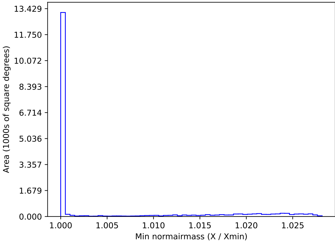
extra_ss_neo4_v3.4_10yrs WFD all bands: Min normairmass
