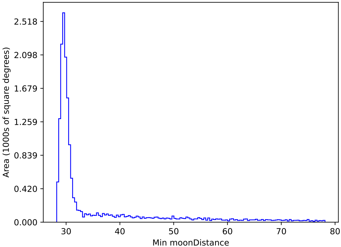
extra_ss_neo4_v3.4_10yrs WFD z band: Min moonDistance
