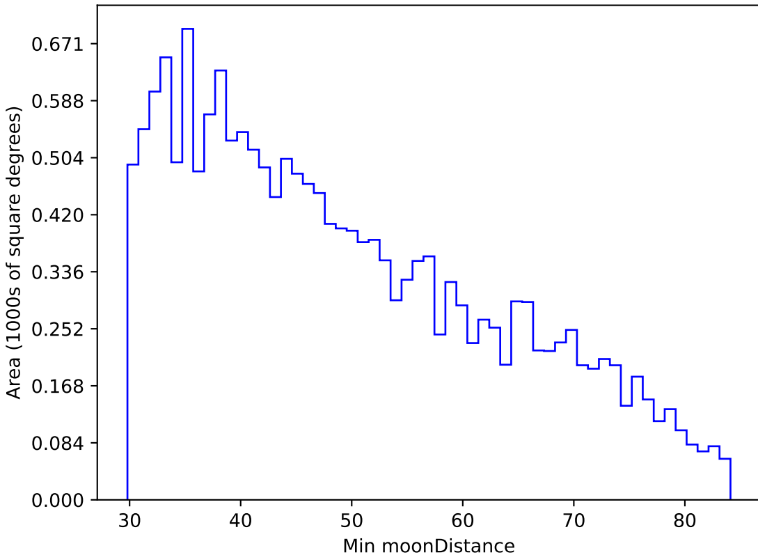
extra_ss_neo4_v3.4_10yrs WFD u band: Min moonDistance
