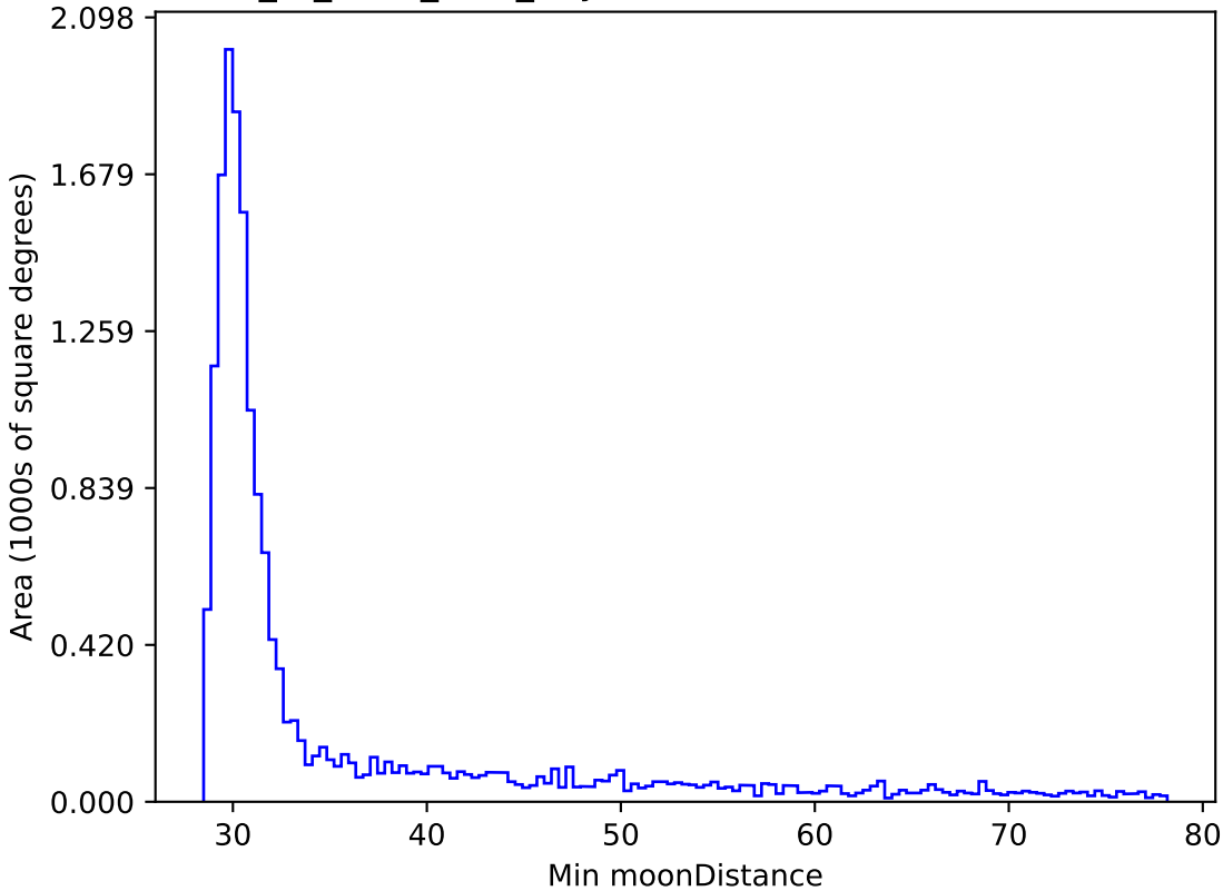
extra_ss_neo4_v3.4_10yrs WFD i band: Min moonDistance
