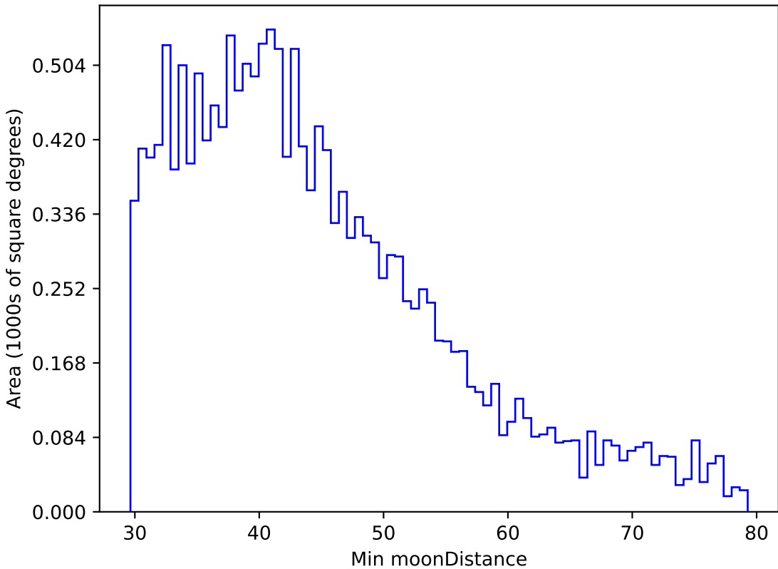
extra_ss_neo4_v3.4_10yrs WFD g band: Min moonDistance
